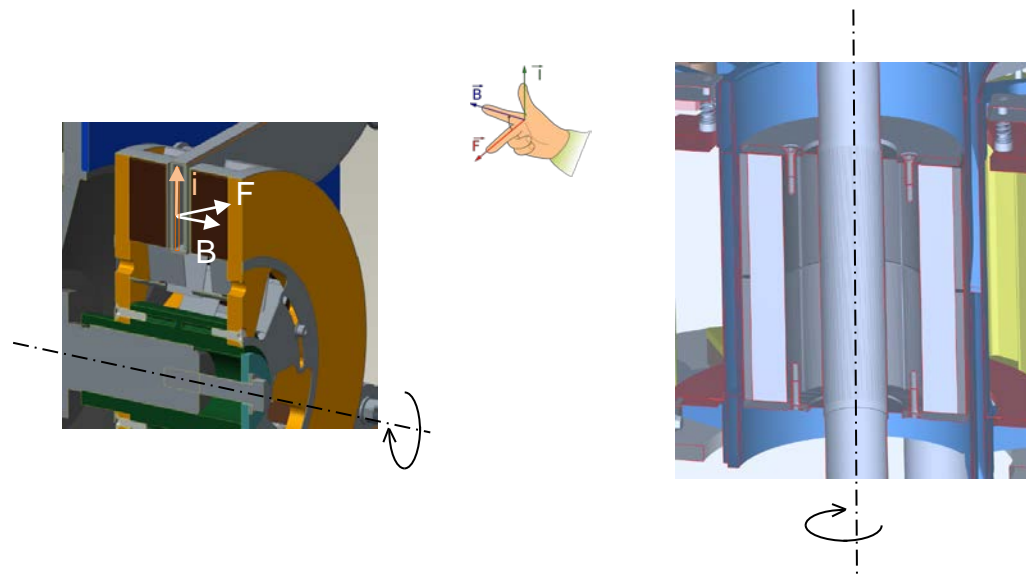
Function principle disc type pump
