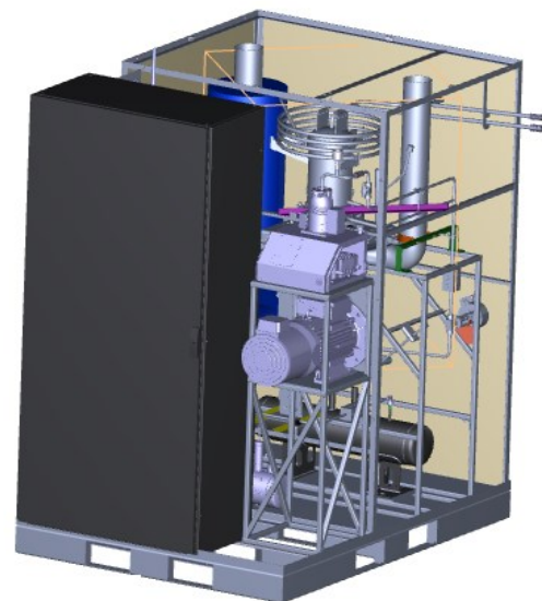
Liquid metal loop under construction in cooperation with Karlsruhe Institute of Technology
